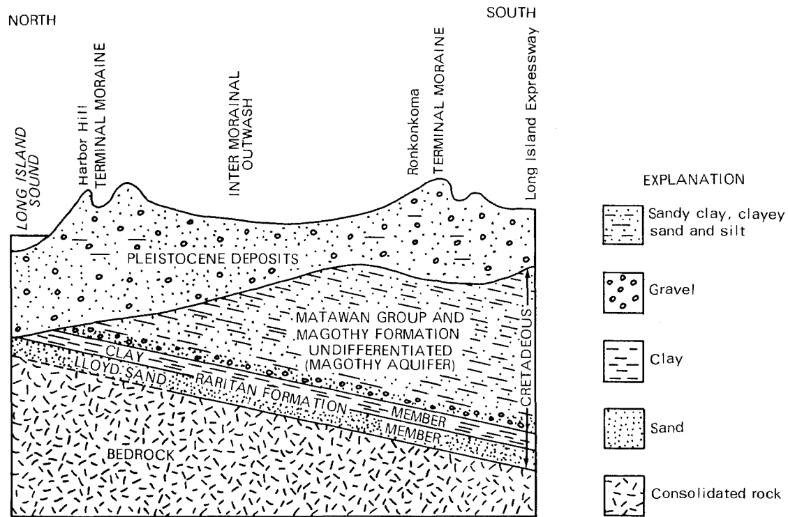
Figure 5.--Generalized geologic cross section of north-central Suffolk County. (From Cohen and others, 1968.)
