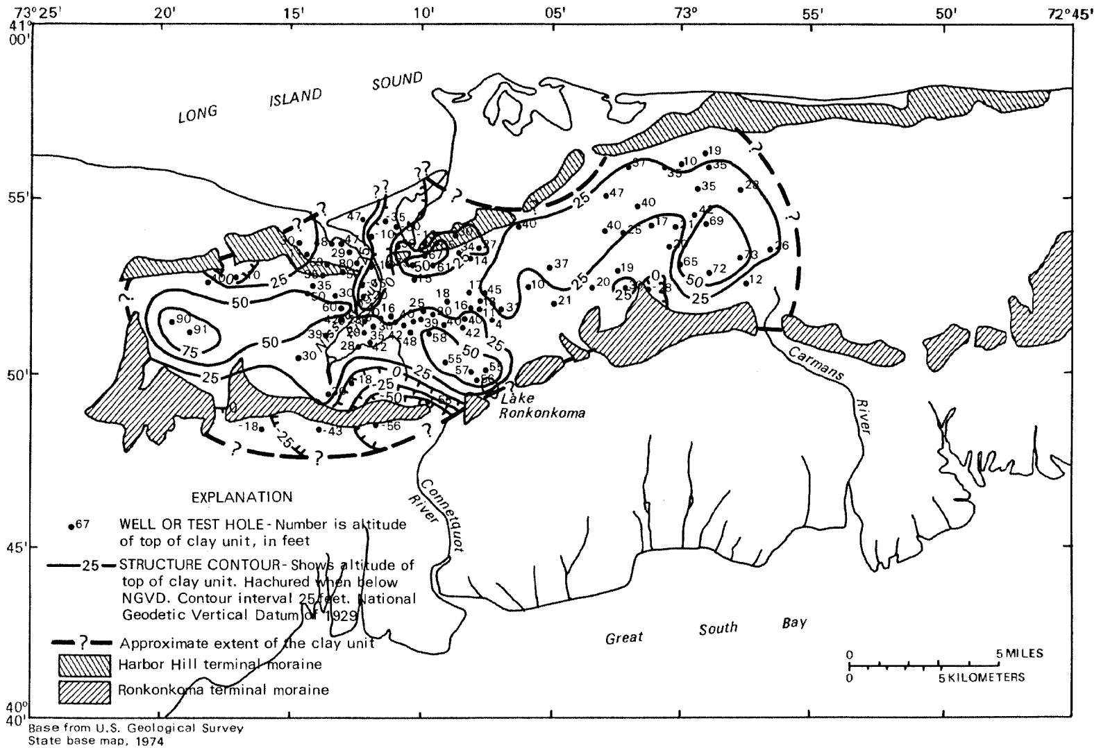
Figure 4.--Altitude of top of clay unit.
