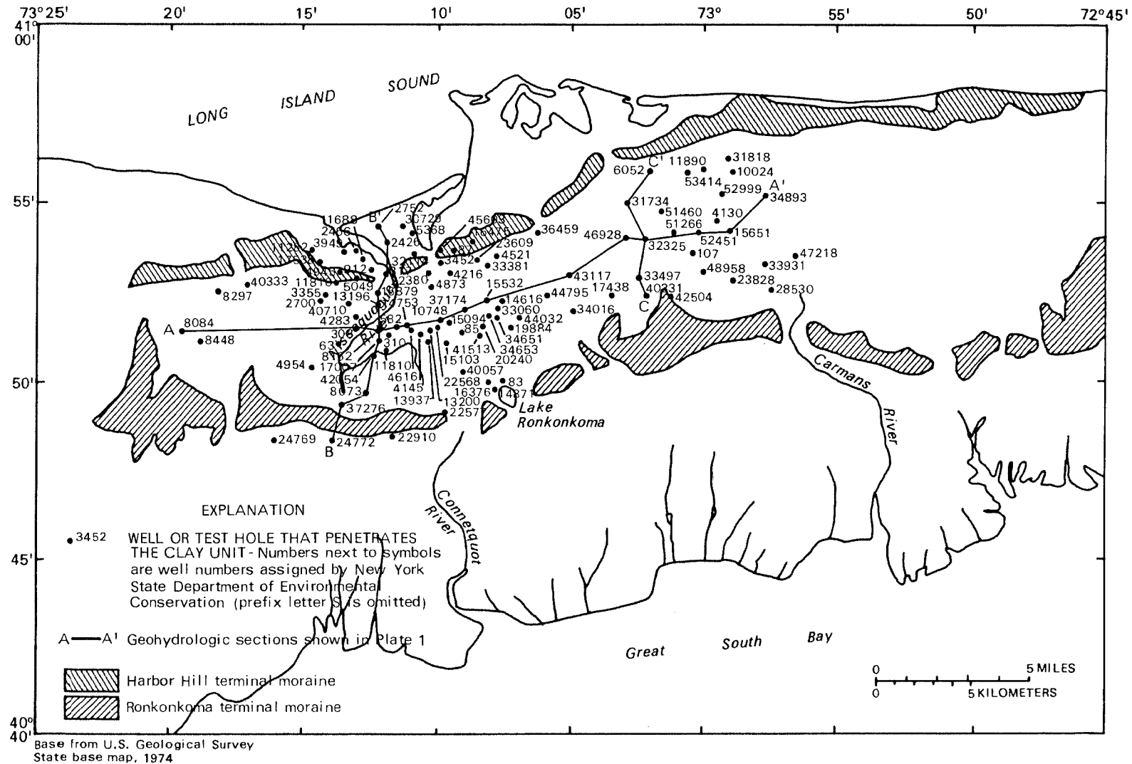
Figure 2.--Location of selected wells penetrating Smithtown Clay. Solid line shows location of geohydrologic cross sections shown in plate 1.
