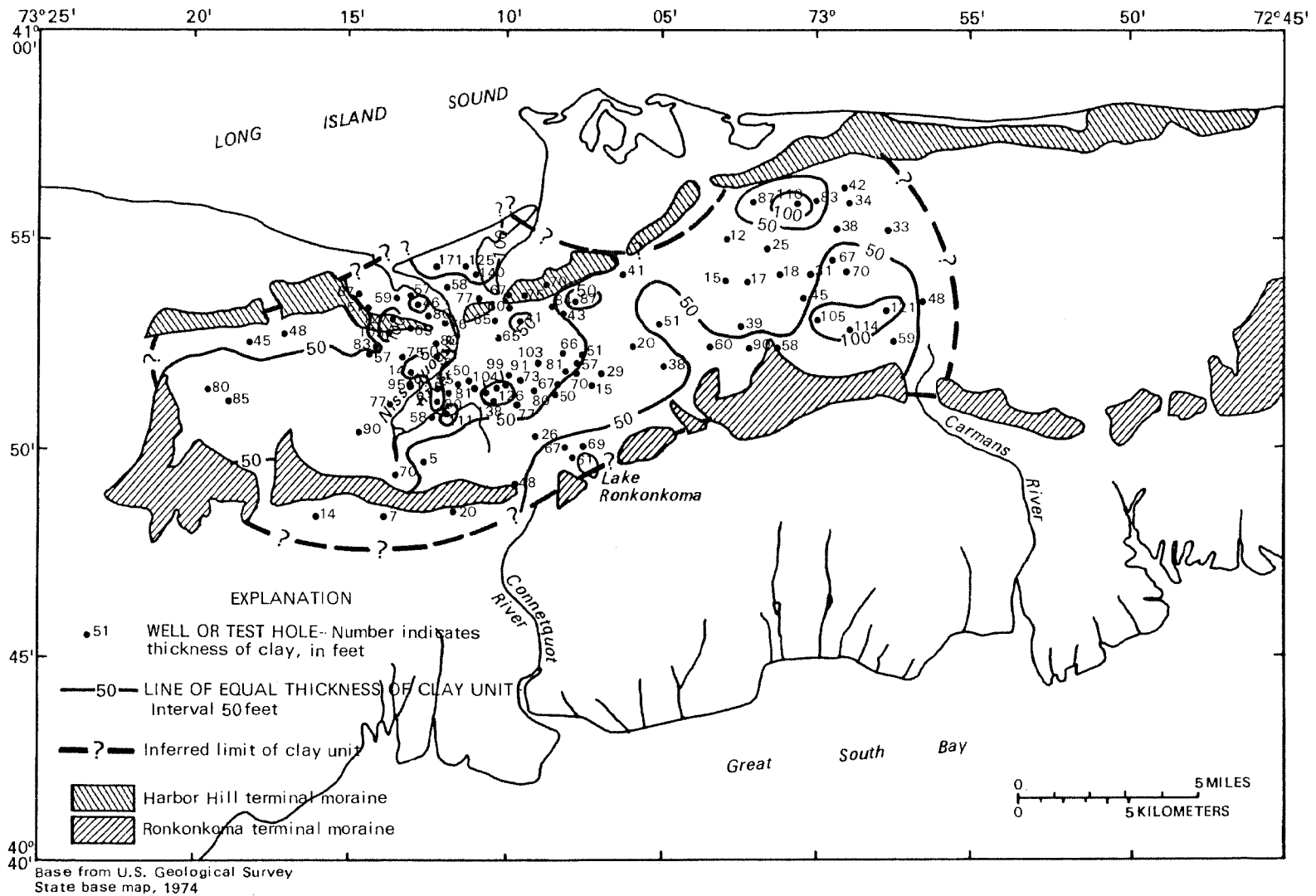
Figure 3.--Thickness of clay unit.
